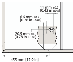
Fig. 1-3 Mounting holes: REC Alpha Panels
