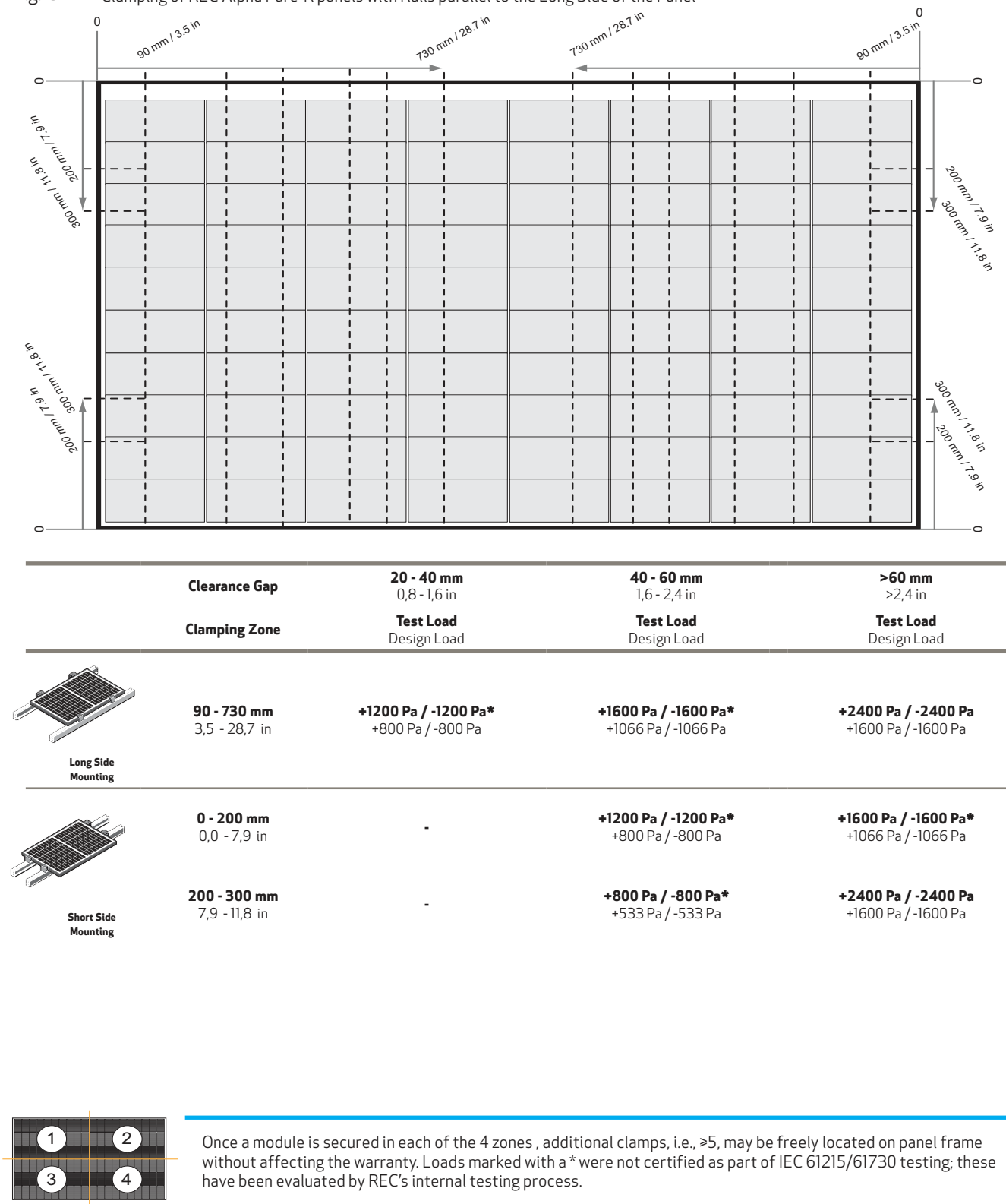
Fig. 3-2 Clamping of REC Alpha Pure-R panels with Rails parallel to the Long Side of the Panel
