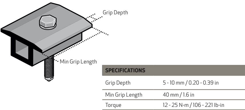
Fig. 1-1 Clamp Specifications
