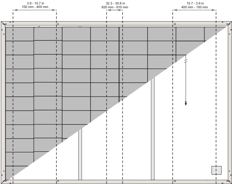
Fig. 4-4 Six-point mounting configuration clamping zones: REC Alpha Pure-RX
