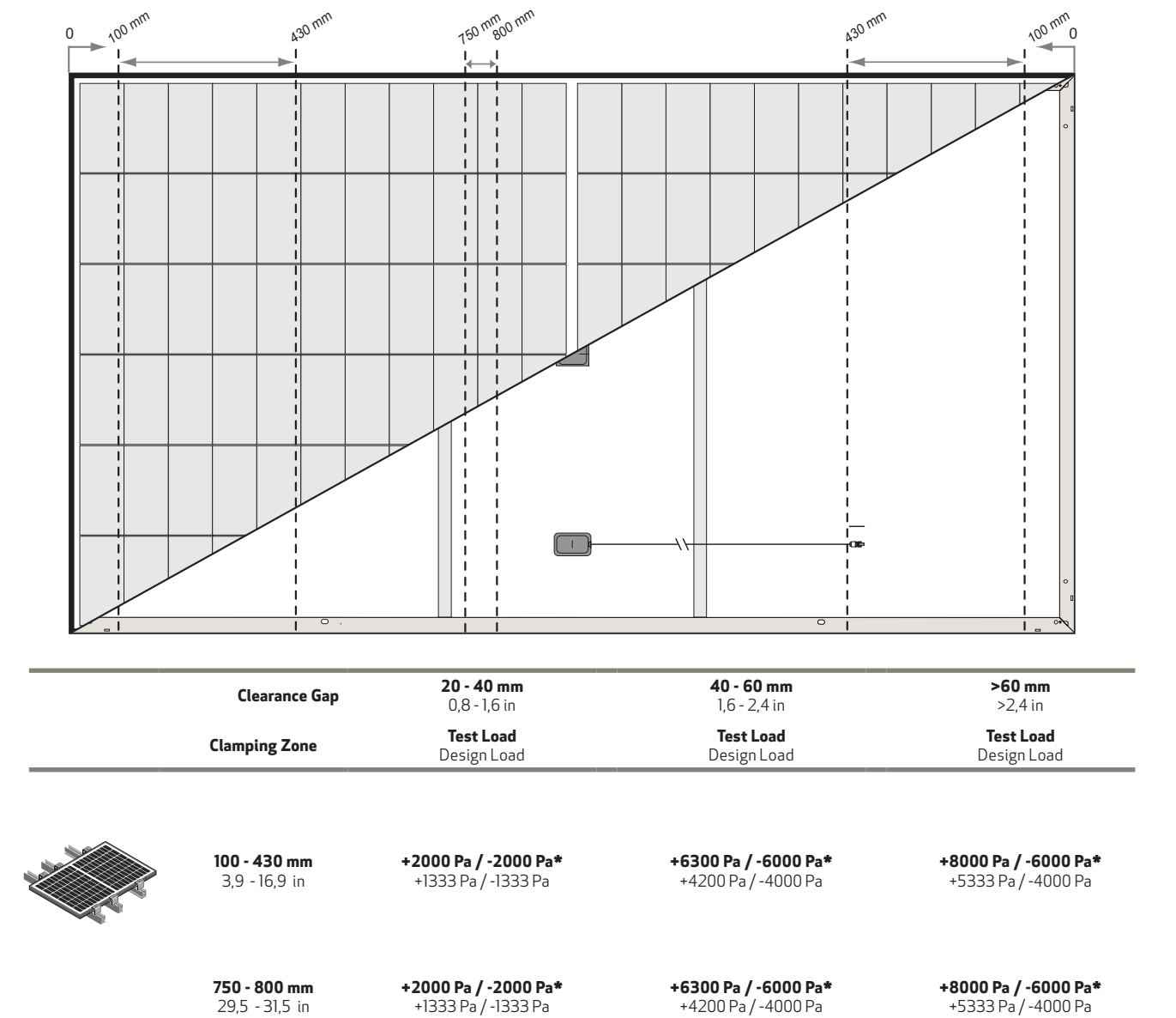
Fig. 2-4 Six-point mounting configuration clamping zones: REC Alpha Pure 2
